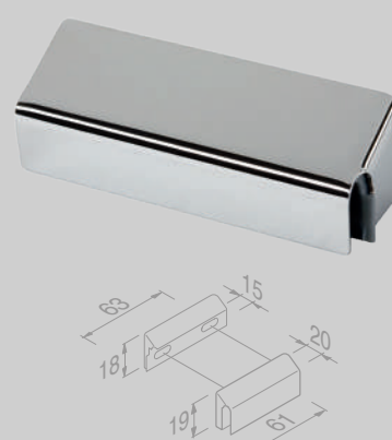
Set verborgen bevestiging* Set concealed fixing* 91697
