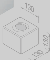
Tissuehouder vrijstaand Tissue dispenser freestanding 911211-02
