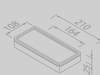
Planket universeel 21 cm Shelf universal 21 cm
