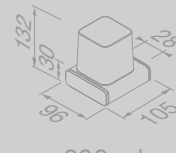
200 ml Zeepdispenser 200 ml met gesatineerd glas Soap dispenser 200 ml with frosted glass
