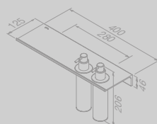
Planchet 40 cm met dispenser multi 200 ml Bathroom shelf 40 cm with dispenser multi 200 ml
