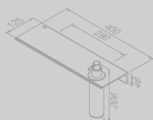
Planchet 40 cm met zeepdispenser 200 ml Bathroom shelf 40 cm with soap dispenser 200 ml
