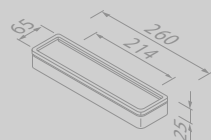
Planket 26 cm Shelf 26 cm
