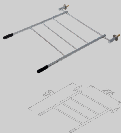
Emmerrooster 40 cm Bucket grating 40 cm
