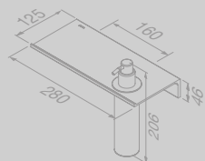
Planchet 28 cm met handdoekhaak en zeepdispenser 200 ml Bathroom shelf 28 cm with towel hook and soap dispenser 200 ml
