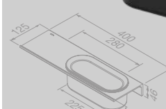
Planchet 40 cm met douchemand 22,5 cm Bathroom shelf 40 cm with shower basket 22,5 cm
